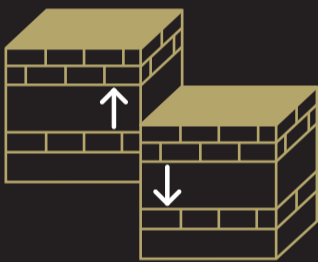
falla vertical
